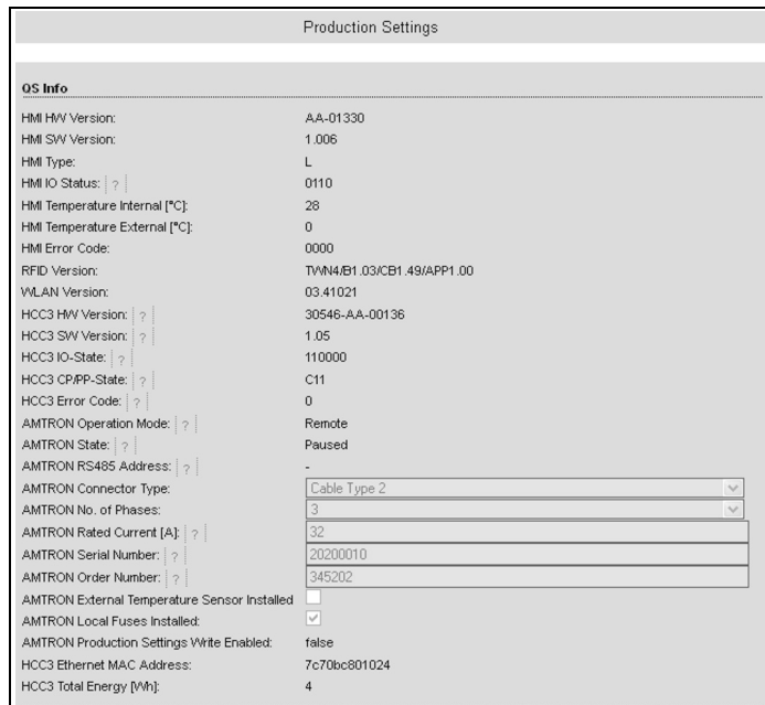
Afb. 16: Menu "Production Settings"
