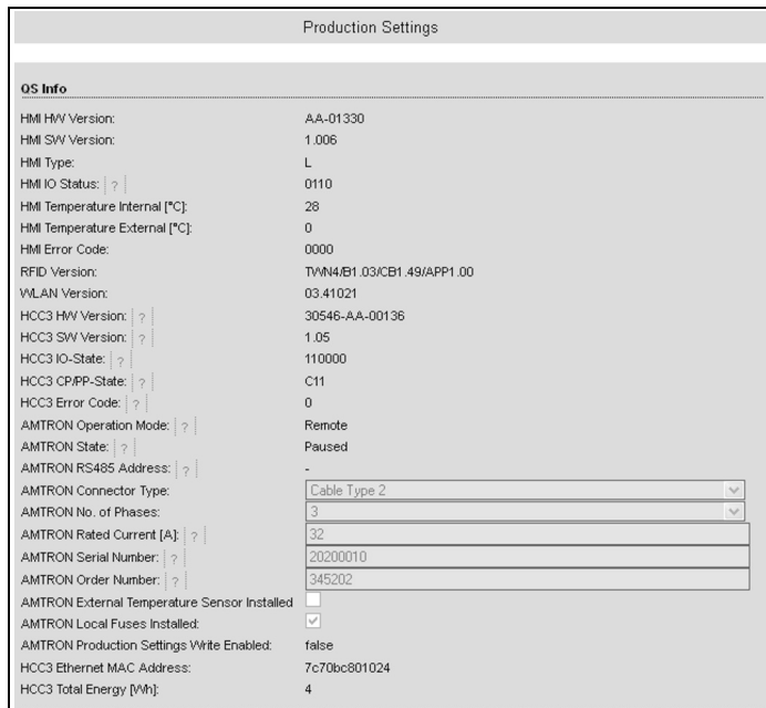
Fig. 16: Menu "Production Settings"
