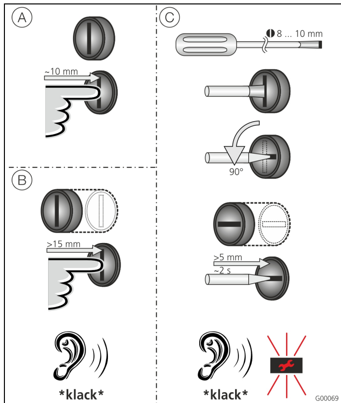
Fig. 8: Multi-function button
